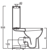
Art. 0250 Vaso monoblocco Soho Soho wc monobloc Art. 0350 Cassetta monoblocco Soho Soho cistern for wc monobloc
